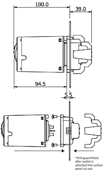
Flush Panel Mount Rear Connect (TBD-R2-IP2X Terminal Block)
