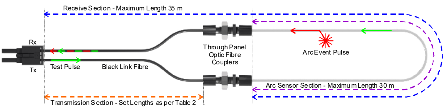
Figure 11: 1S40 Component Function and Installation Limitations
